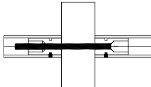
Back to Back Timber Fix
